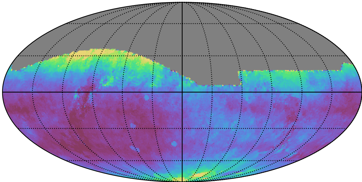
too_elab_r8_d3_gz_v3.4_10yrs All sky r band: Median seeingEff
