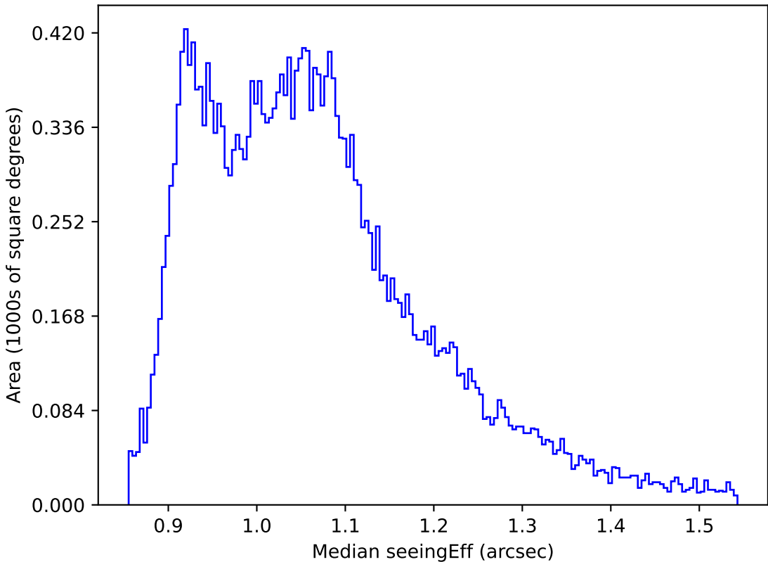
too_elab_r8_d3_gz_v3.4_10yrs All sky r band: Median seeingEff
