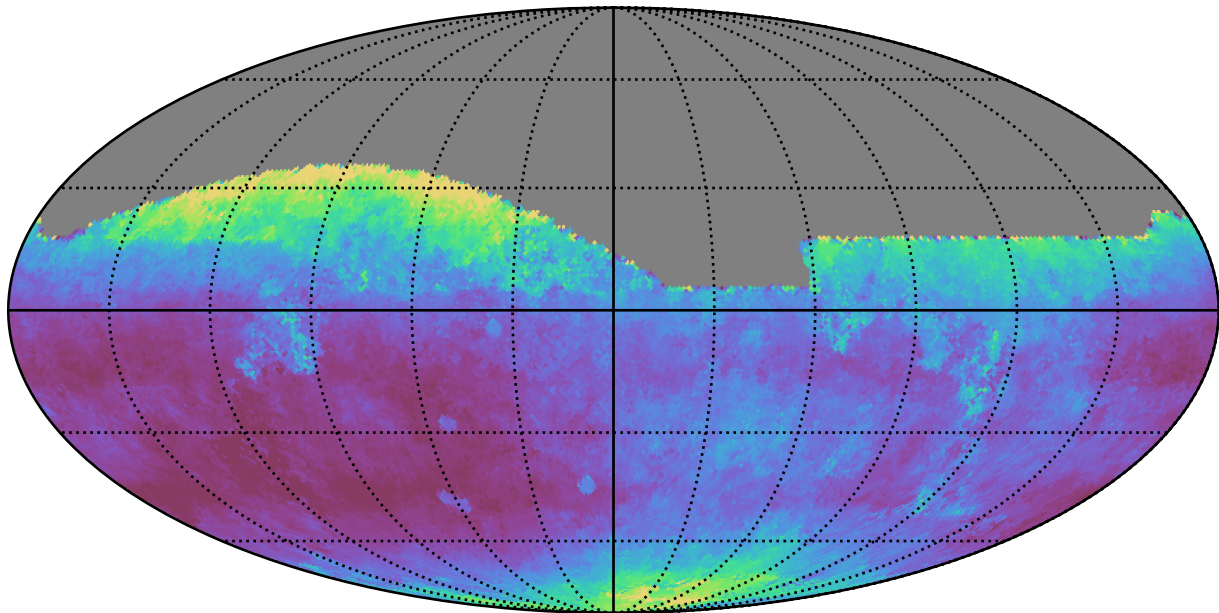
too_elab_r8_d3_gz_v3.4_10yrs All sky i band: Median seeingEff
