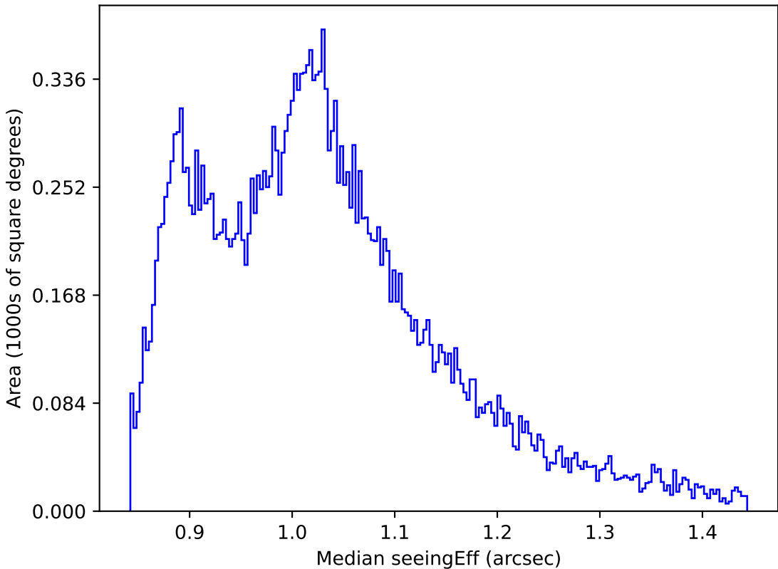
too_elab_r8_d3_gz_v3.4_10yrs All sky i band: Median seeingEff
