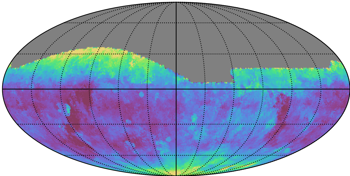
too_elab_r8_d3_gz_v3.4_10yrs All sky g band: Median seeingEff
