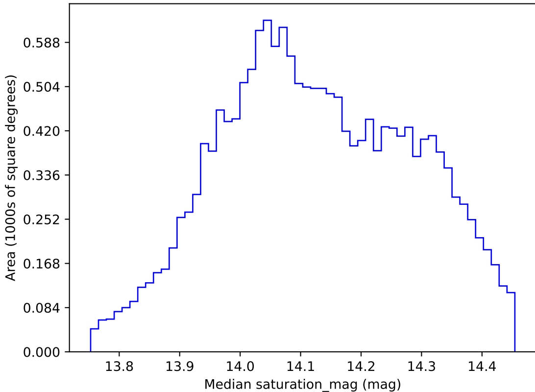
too_elab_r8_d3_gz_v3.4_10yrs WFD z band: Median saturation_mag
