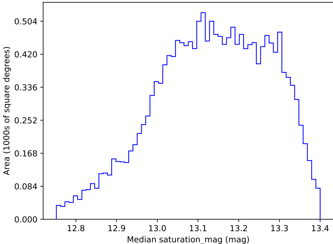
too_elab_r8_d3_gz_v3.4_10yrs WFD y band: Median saturation_mag
