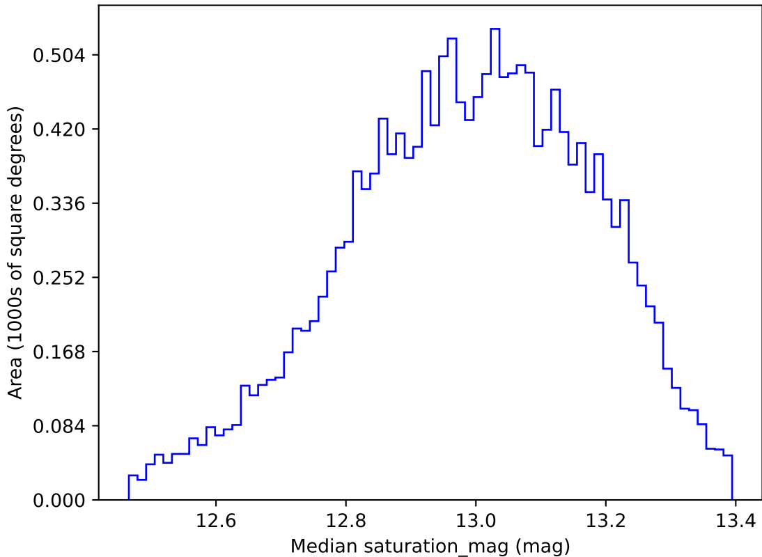
too_elab_r8_d3_gz_v3.4_10yrs WFD u band: Median saturation_mag
