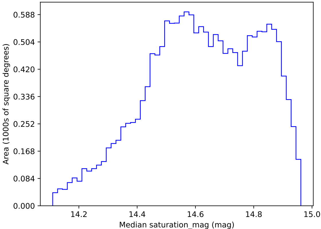
too_elab_r8_d3_gz_v3.4_10yrs WFD r band: Median saturation_mag
