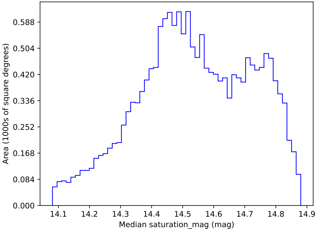
too_elab_r8_d3_gz_v3.4_10yrs WFD i band: Median saturation_mag
