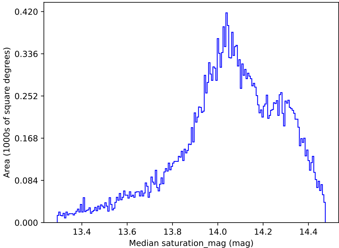
too_elab_r8_d3_gz_v3.4_10yrs All sky z band: Median saturation_mag
