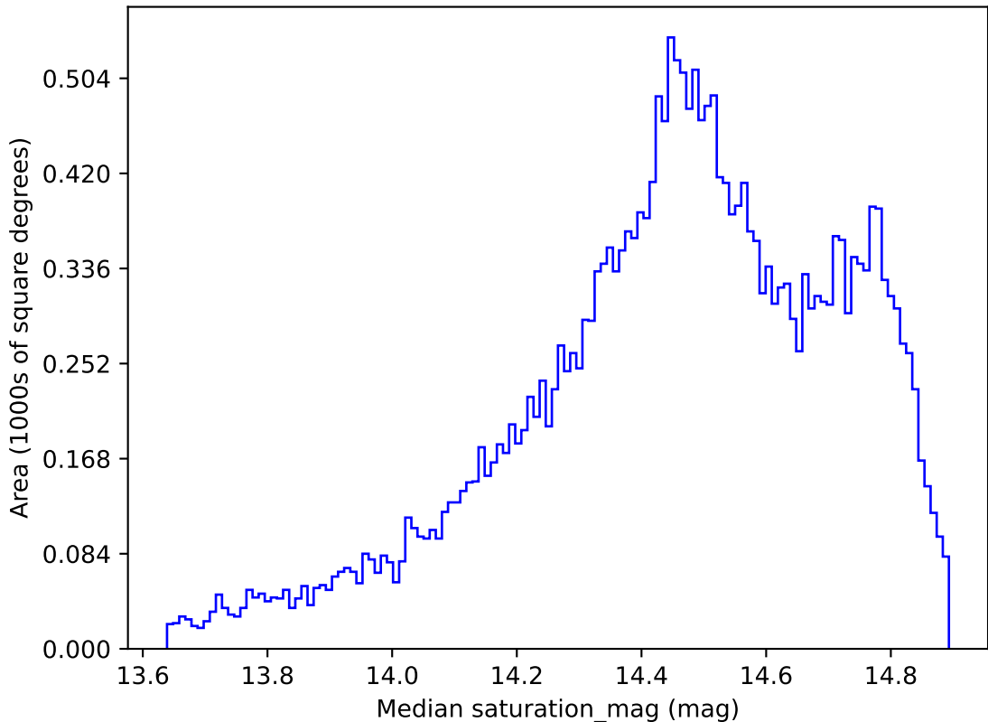
too_elab_r8_d3_gz_v3.4_10yrs All sky i band: Median saturation_mag
