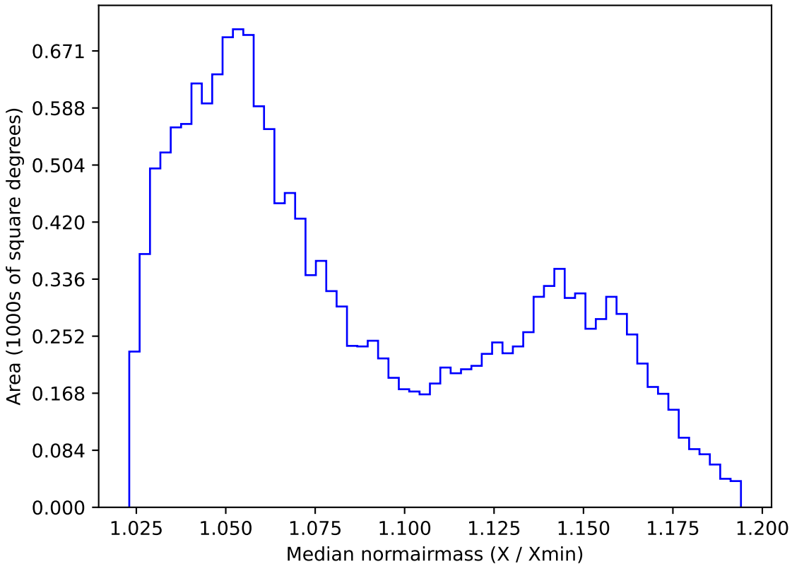
too_elab_r8_d3_gz_v3.4_10yrs WFD z band: Median normairmass
