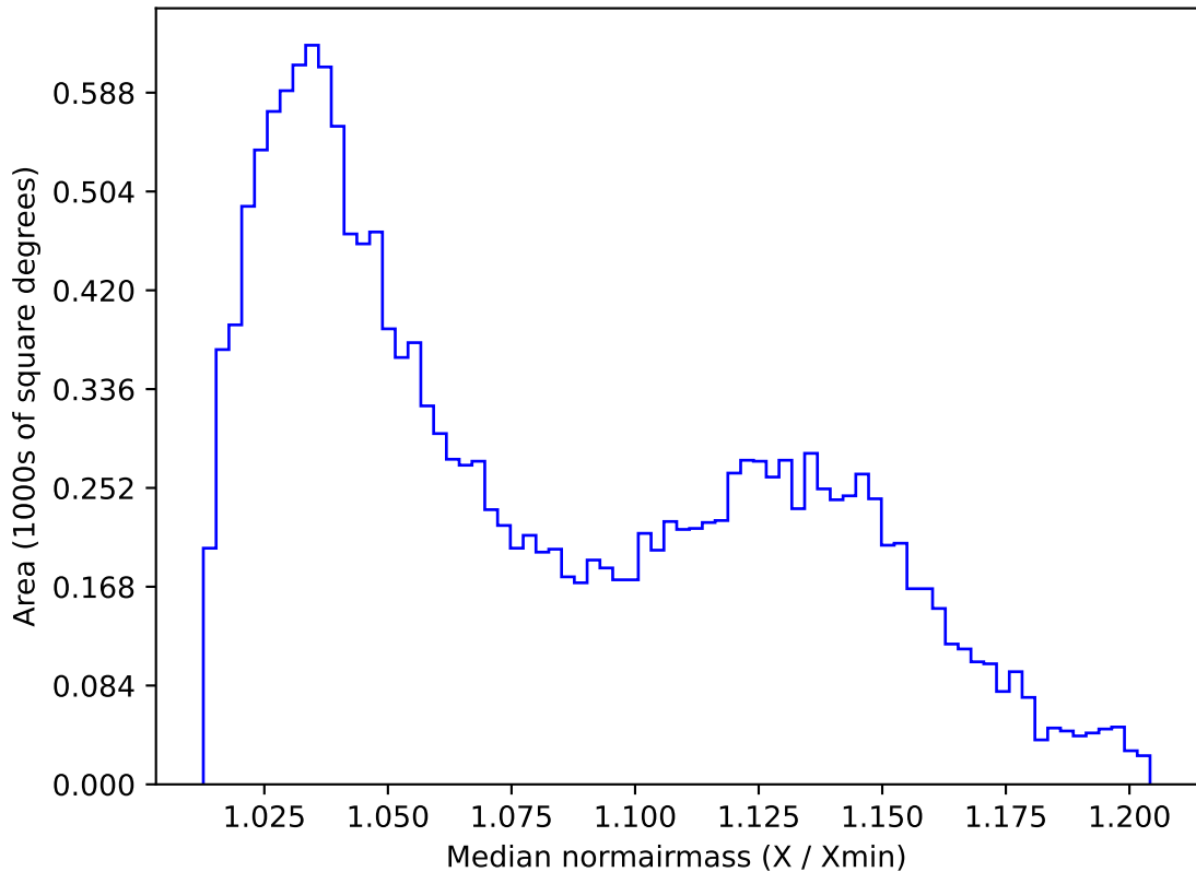
too_elab_r8_d3_gz_v3.4_10yrs WFD u band: Median normairmass
