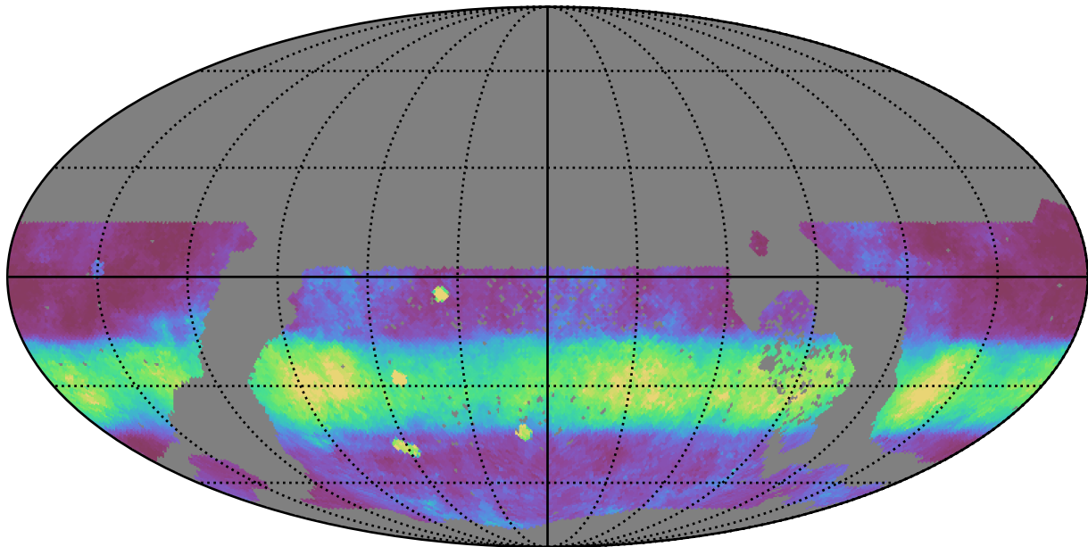
too_elab_r8_d3_gz_v3.4_10yrs WFD r band: Median normairmass
