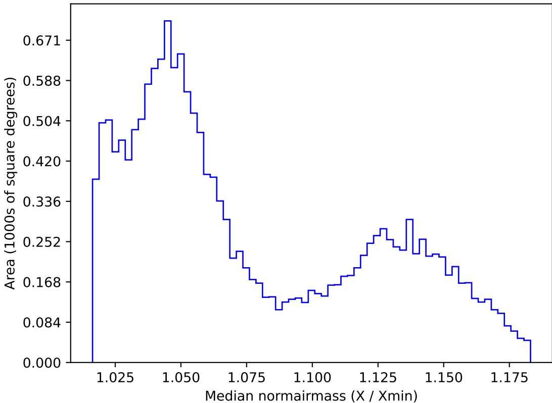
too_elab_r8_d3_gz_v3.4_10yrs WFD r band: Median normairmass
