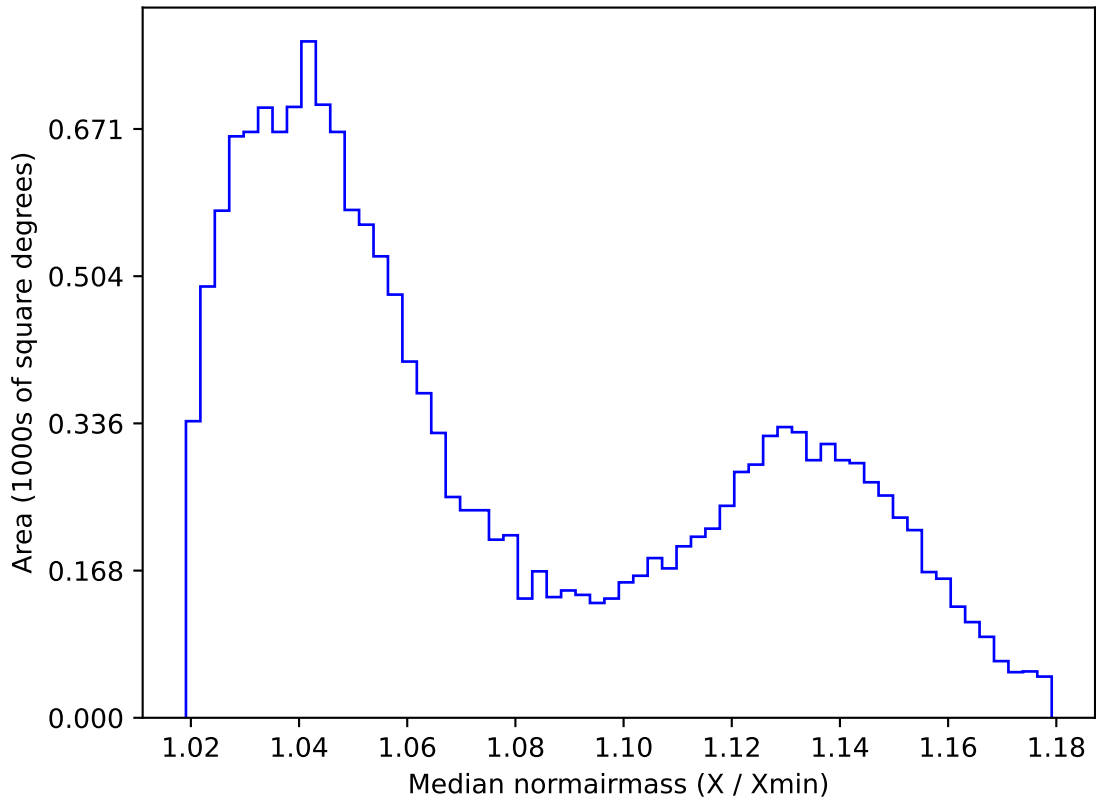
too_elab_r8_d3_gz_v3.4_10yrs WFD i band: Median normairmass
