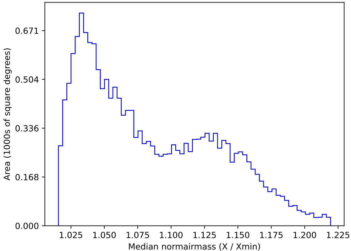
too_elab_r8_d3_gz_v3.4_10yrs WFD g band: Median normairmass
