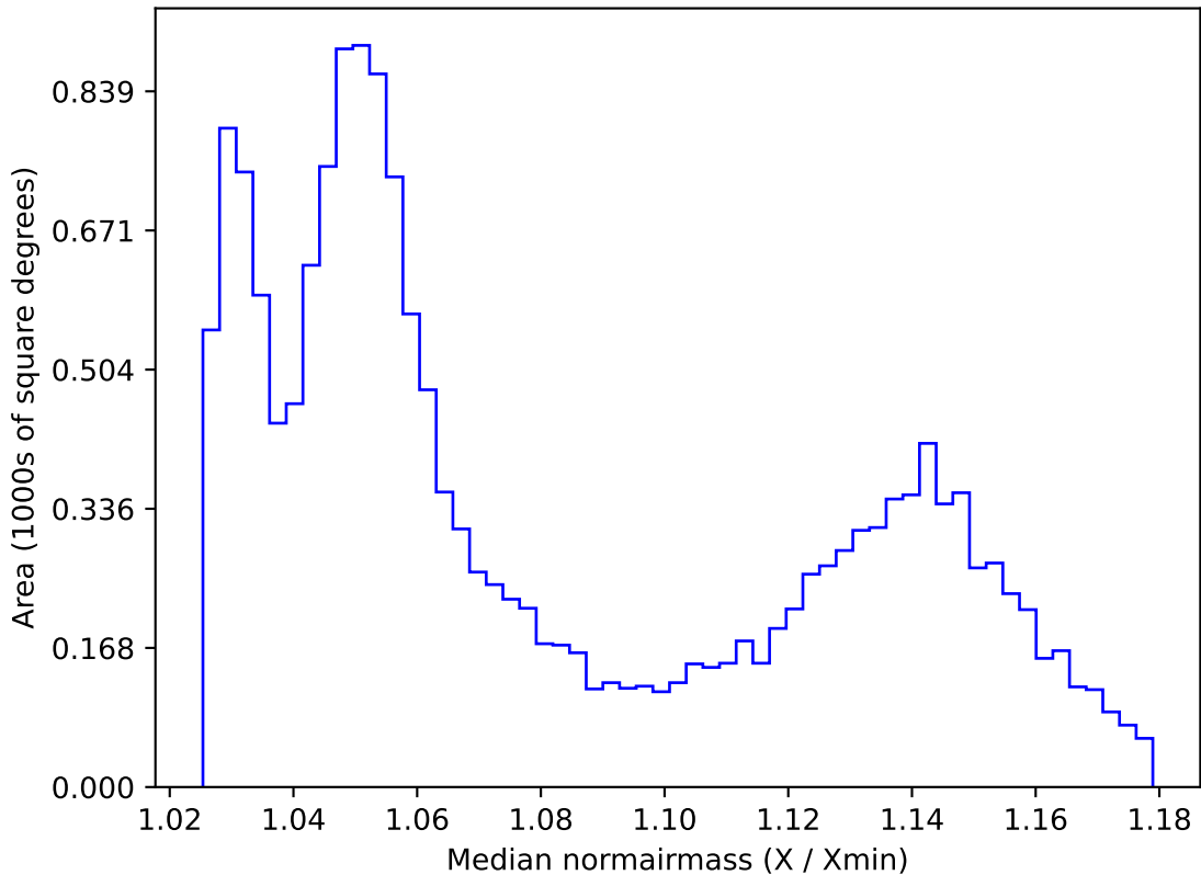
too_elab_r8_d3_gz_v3.4_10yrs WFD all bands: Median normairmass
