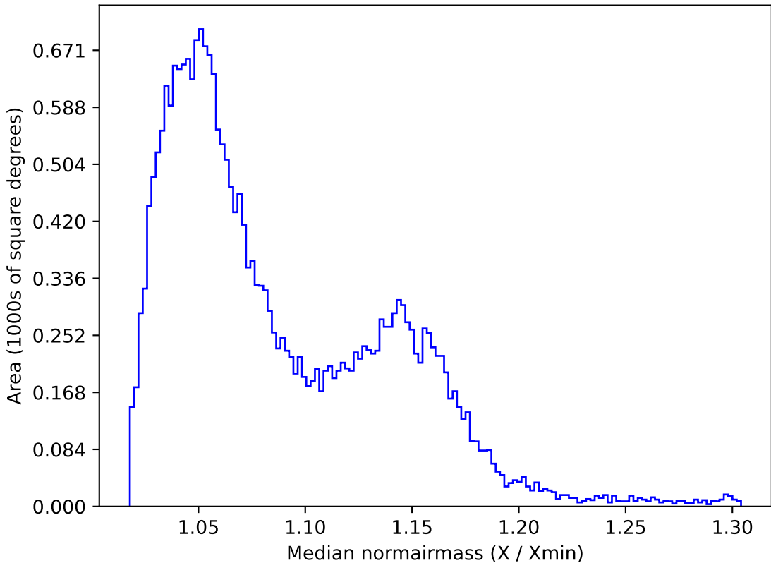
too_elab_r8_d3_gz_v3.4_10yrs All sky z band: Median normairmass
