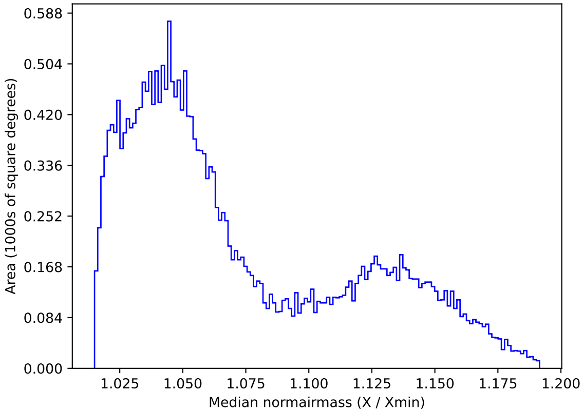
too_elab_r8_d3_gz_v3.4_10yrs All sky r band: Median normairmass
