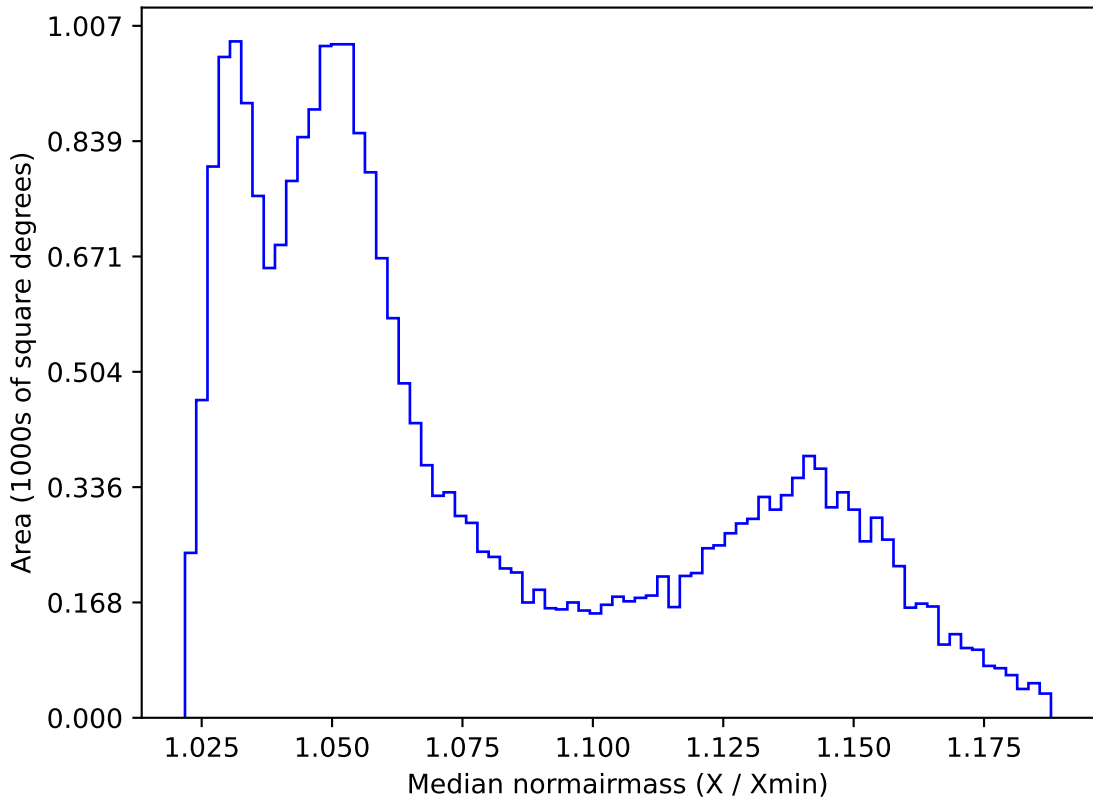
too_elab_r8_d3_gz_v3.4_10yrs All sky all bands: Median normairmass
