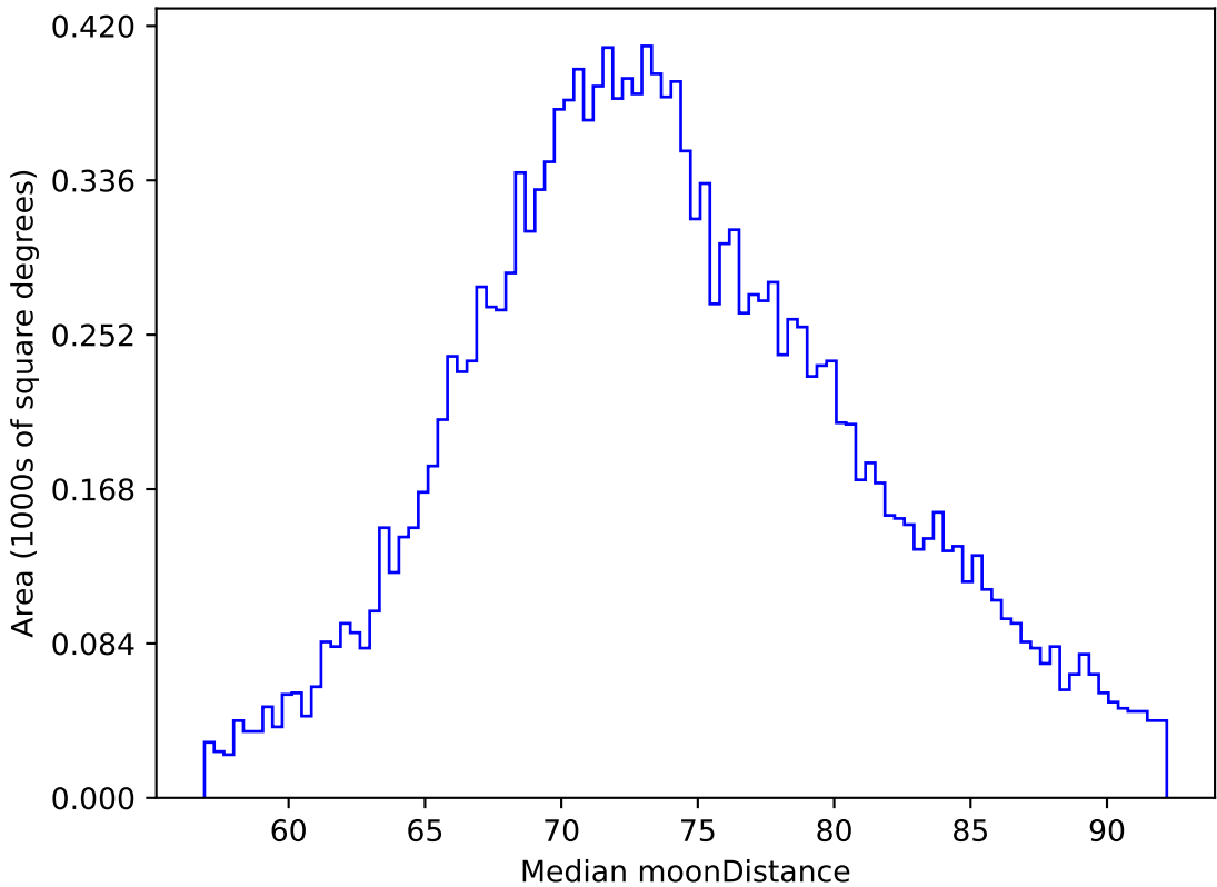
too_elab_r8_d3_gz_v3.4_10yrs WFD z band: Median moonDistance
