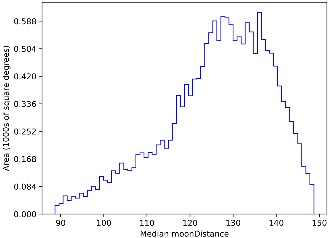
too_elab_r8_d3_gz_v3.4_10yrs WFD u band: Median moonDistance
