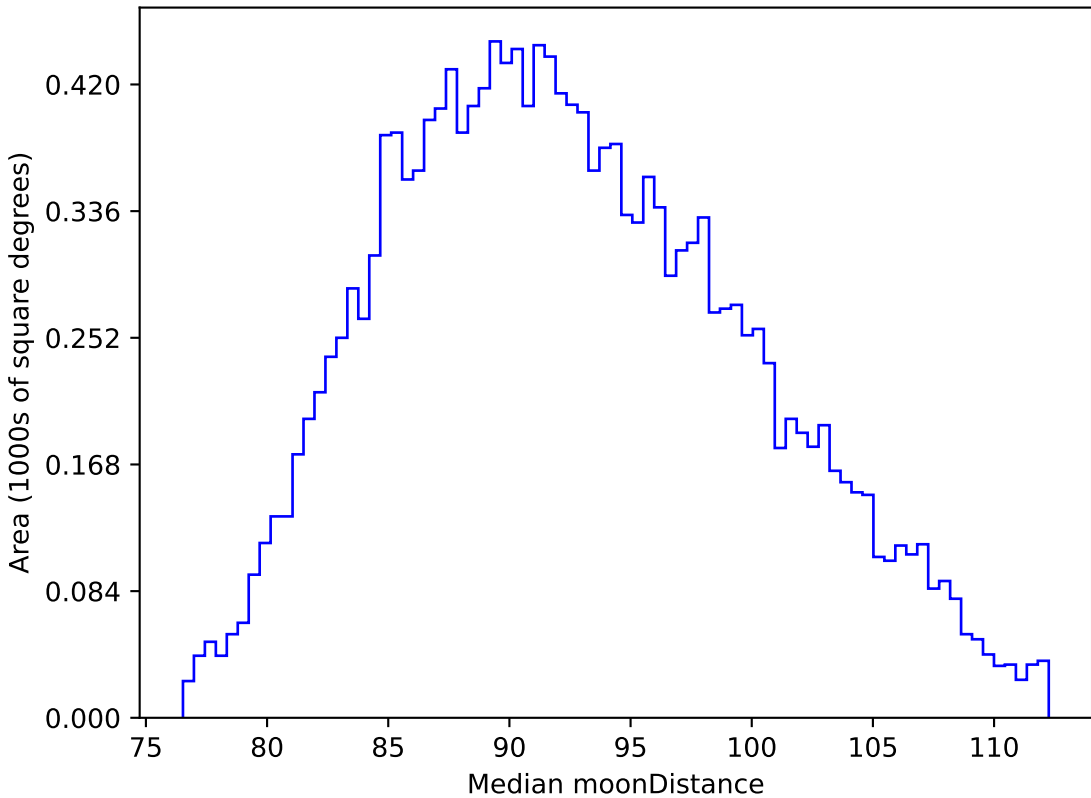
too_elab_r8_d3_gz_v3.4_10yrs WFD i band: Median moonDistance
