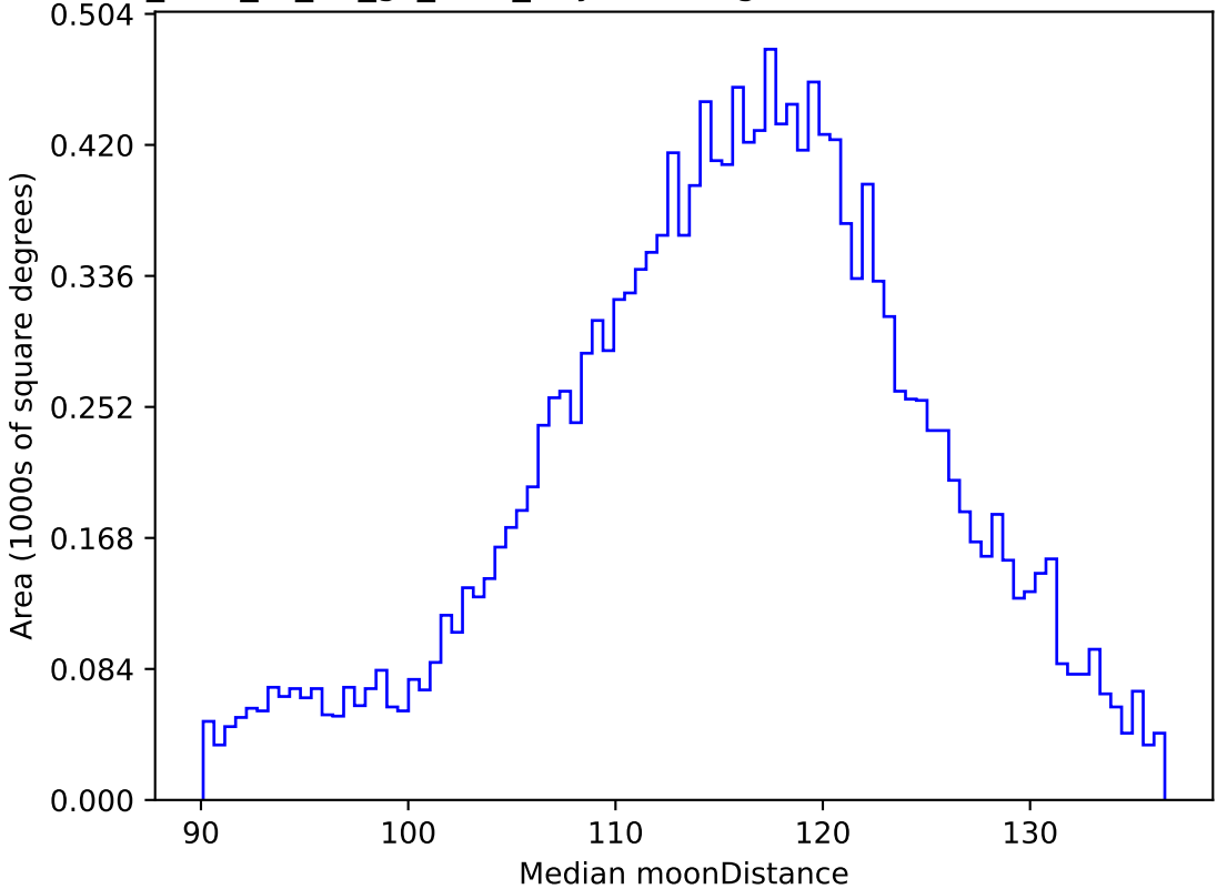
too_elab_r8_d3_gz_v3.4_10yrs WFD g band: Median moonDistance
