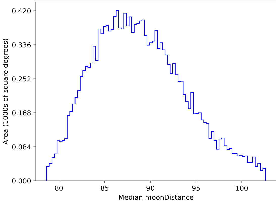
too_elab_r8_d3_gz_v3.4_10yrs WFD all bands: Median moonDistance
