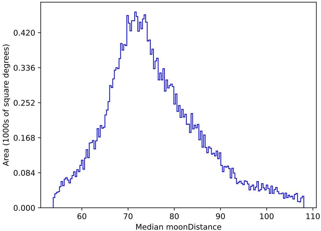
too_elab_r8_d3_gz_v3.4_10yrs All sky z band: Median moonDistance
