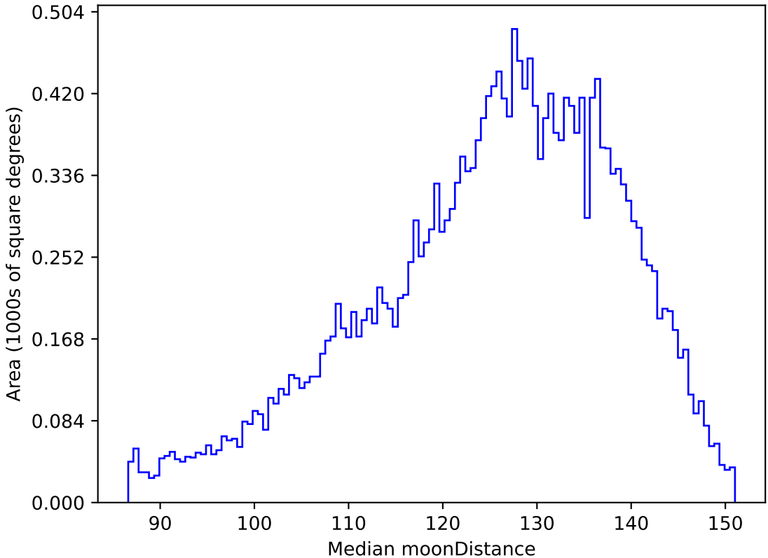
too_elab_r8_d3_gz_v3.4_10yrs All sky u band: Median moonDistance
