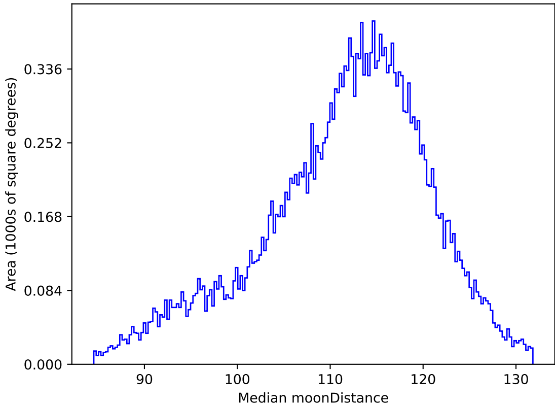
too_elab_r8_d3_gz_v3.4_10yrs All sky r band: Median moonDistance
