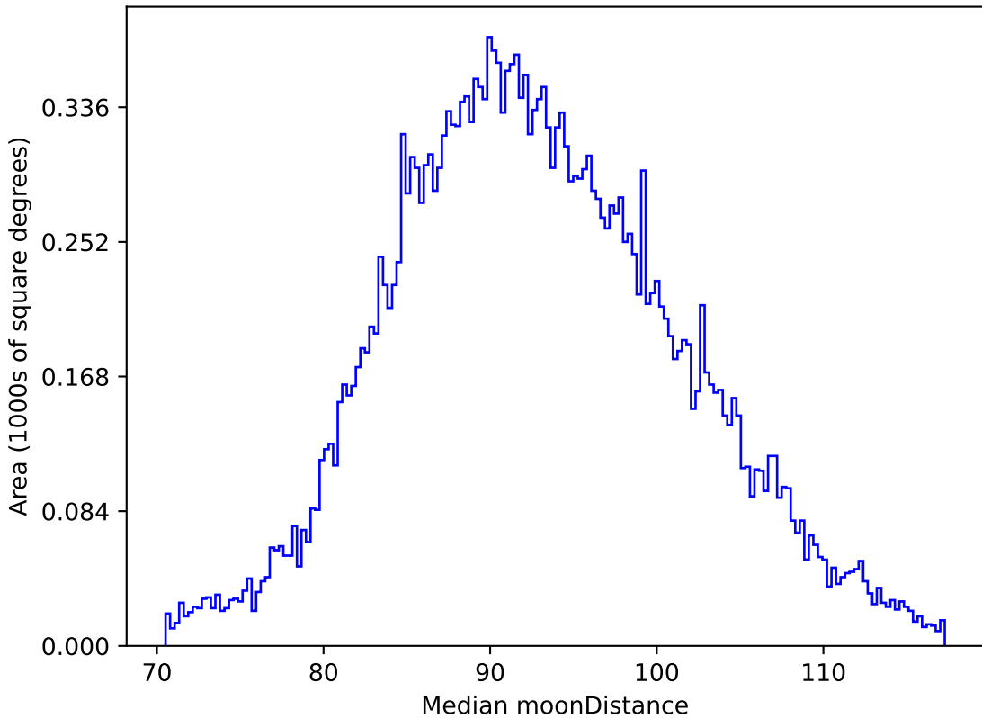
too_elab_r8_d3_gz_v3.4_10yrs All sky i band: Median moonDistance
