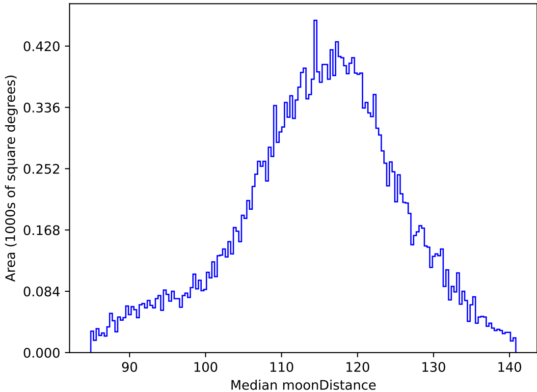
too_elab_r8_d3_gz_v3.4_10yrs All sky g band: Median moonDistance
