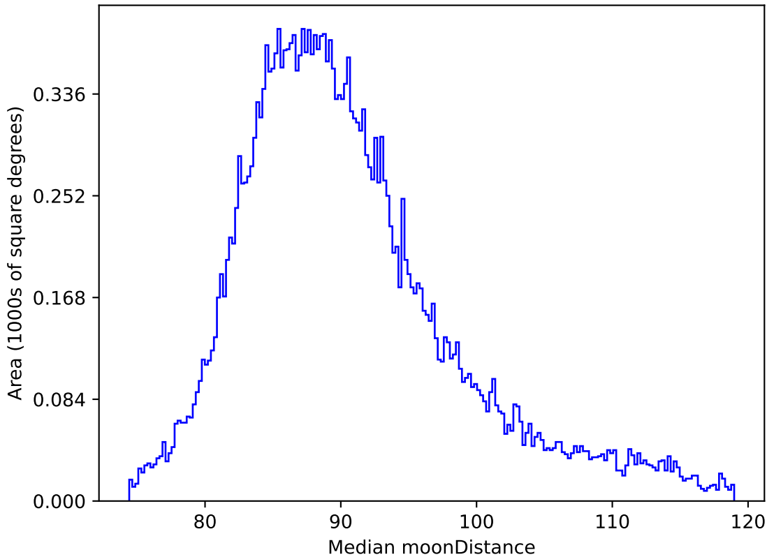
too_elab_r8_d3_gz_v3.4_10yrs All sky all bands: Median moonDistance
