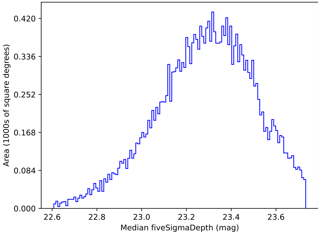
too_elab_r8_d3_gz_v3.4_10yrs Yr 1 u band: Median fiveSigmaDepth
