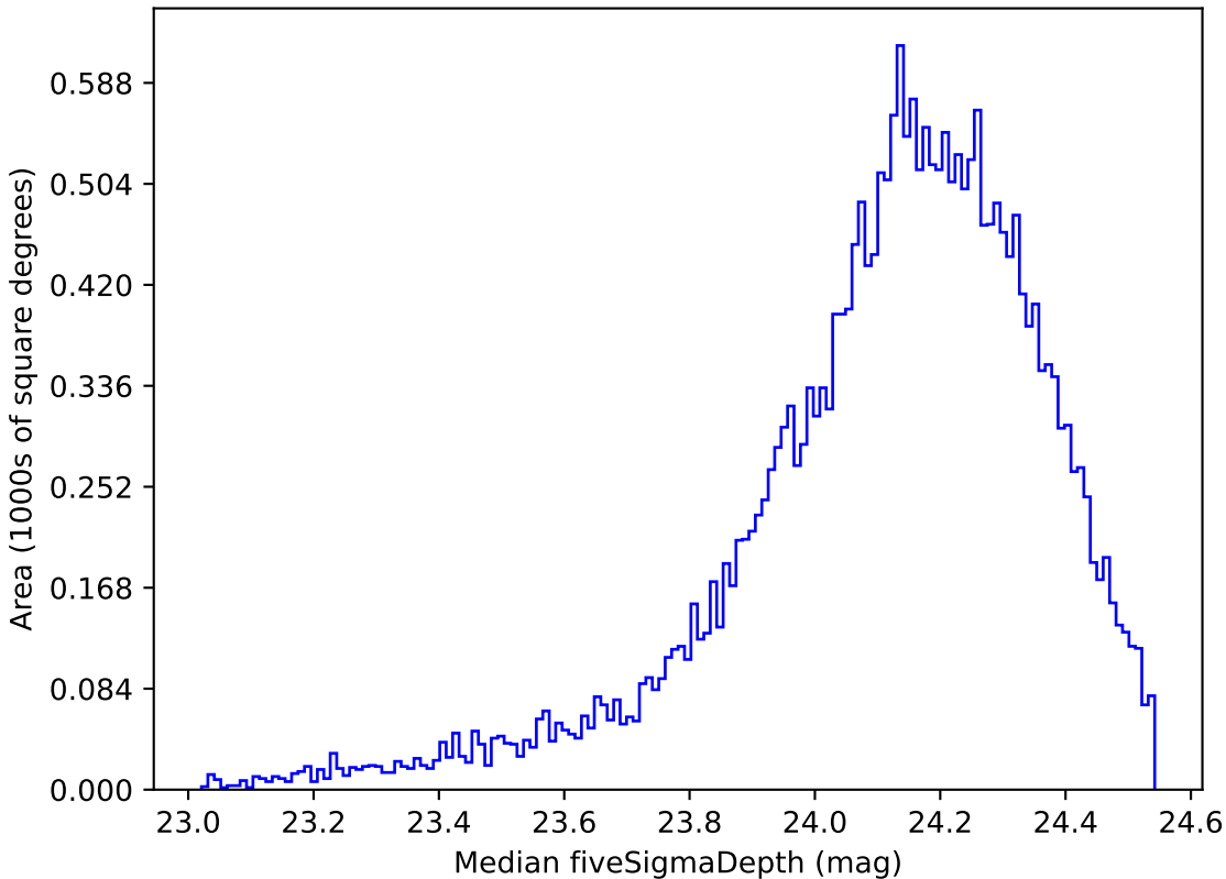
too_elab_r8_d3_gz_v3.4_10yrs Yr 1 r band: Median fiveSigmaDepth
