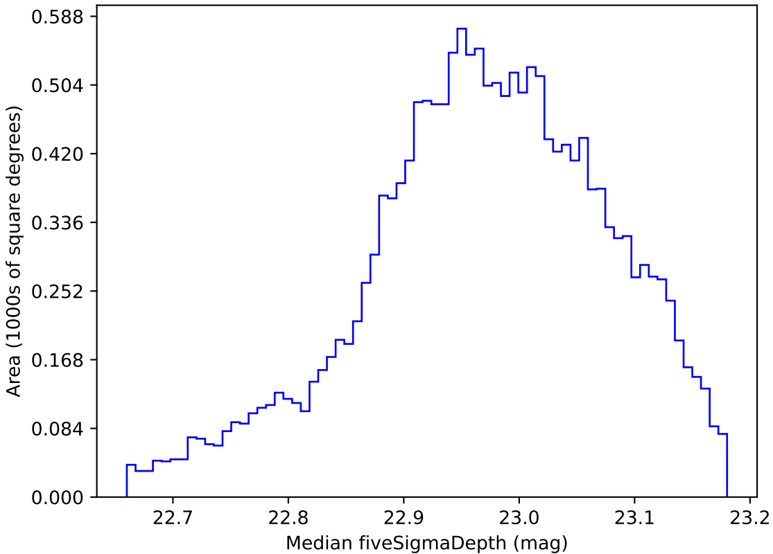
too_elab_r8_d3_gz_v3.4_10yrs WFD z band: Median fiveSigmaDepth
