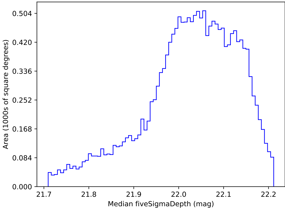
too_elab_r8_d3_gz_v3.4_10yrs WFD y band: Median fiveSigmaDepth
