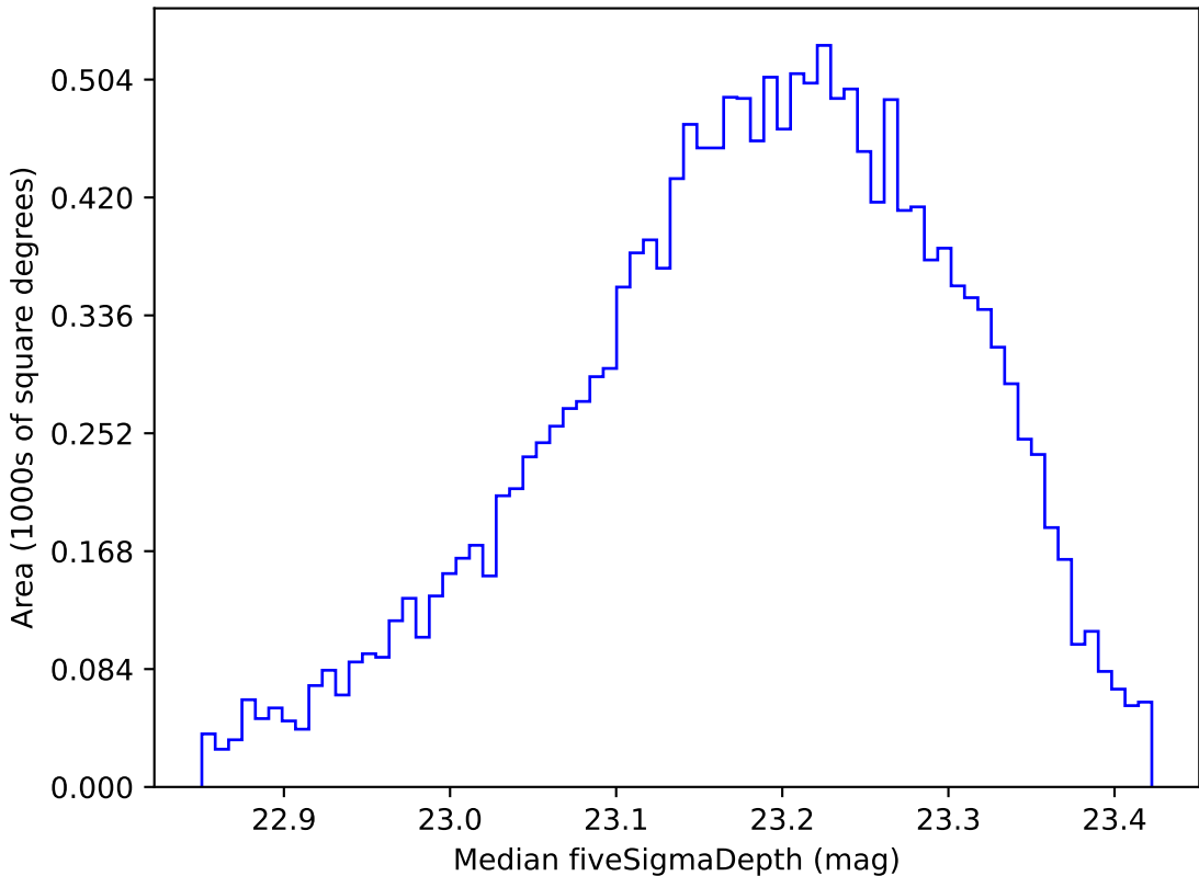
too_elab_r8_d3_gz_v3.4_10yrs WFD u band: Median fiveSigmaDepth
