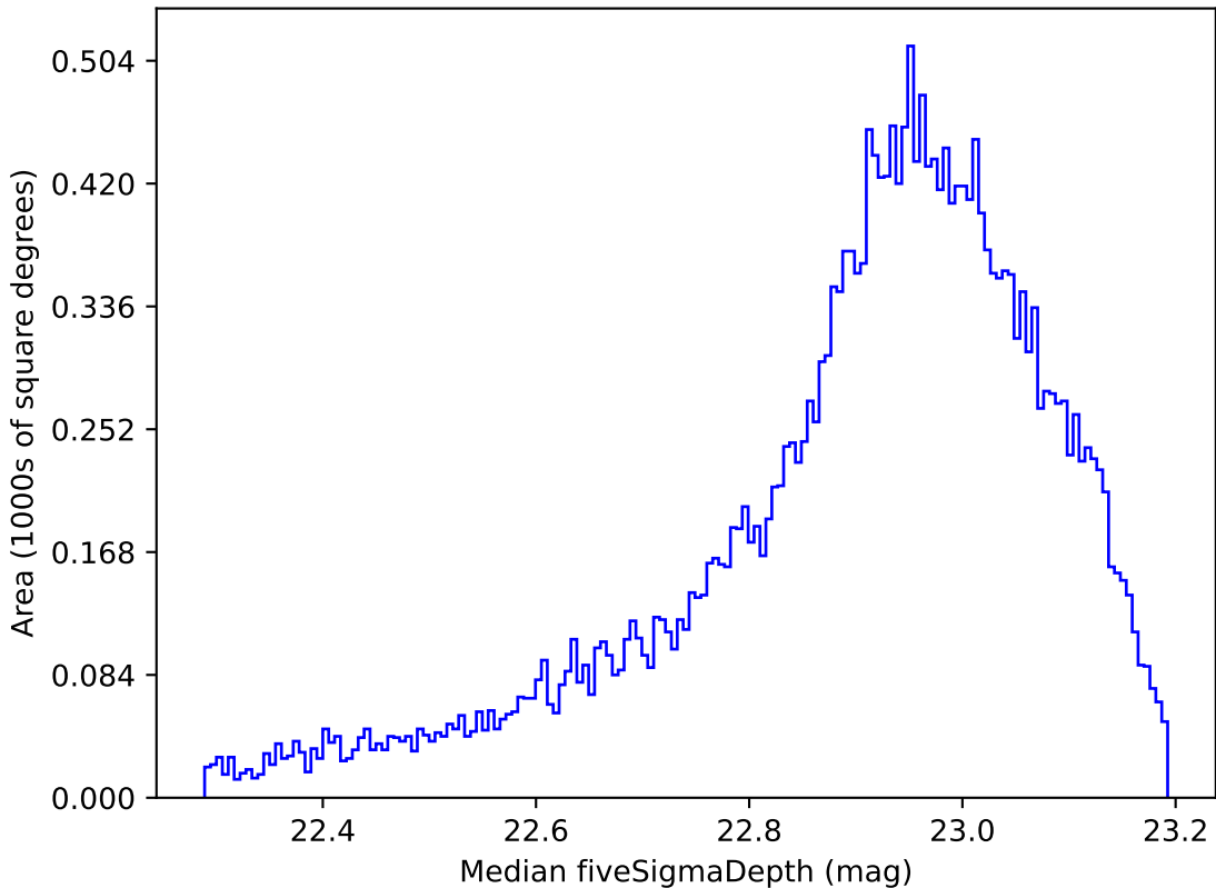
too_elab_r8_d3_gz_v3.4_10yrs All sky z band: Median fiveSigmaDepth
