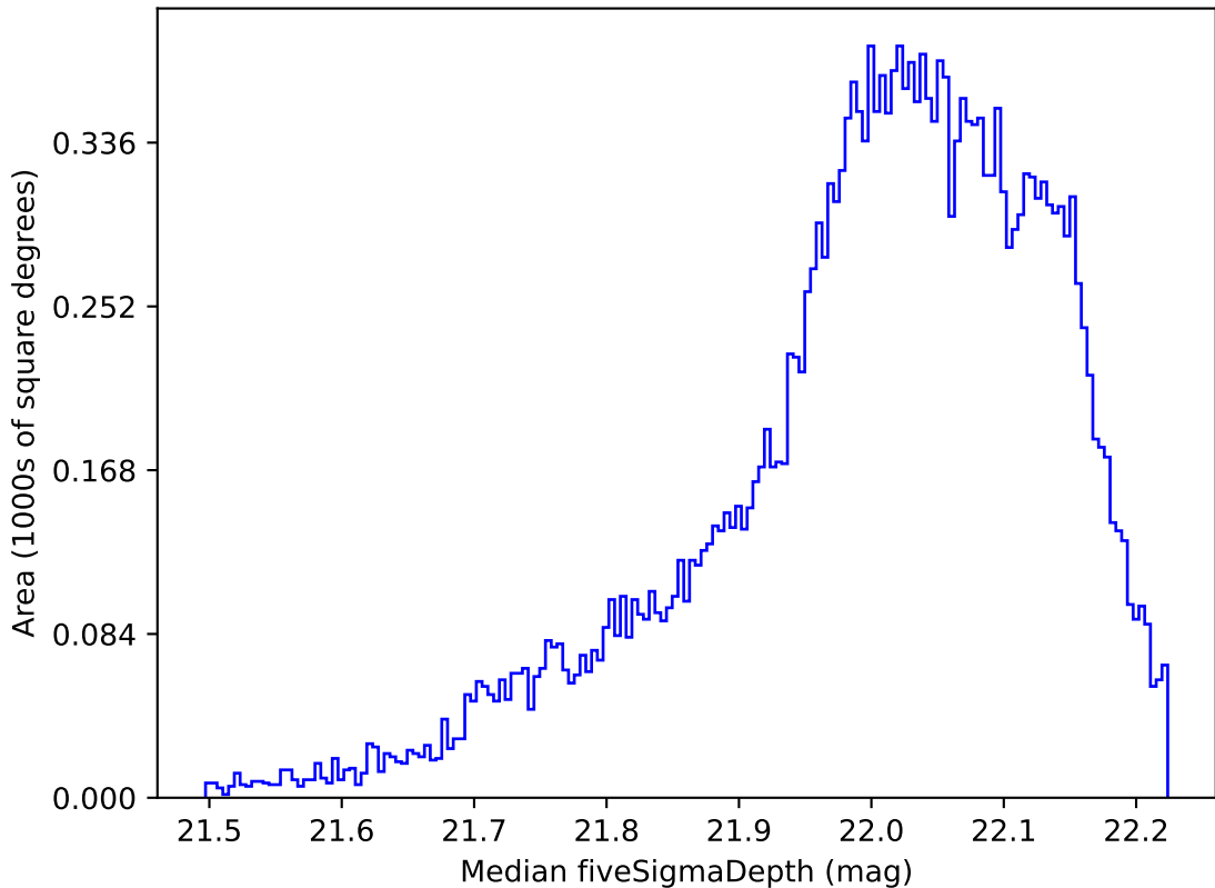
too_elab_r8_d3_gz_v3.4_10yrs All sky y band: Median fiveSigmaDepth
