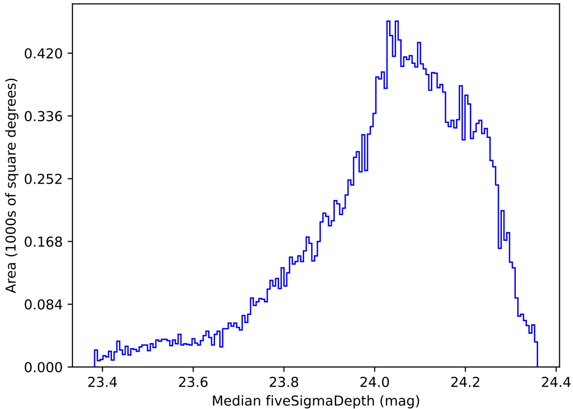
too_elab_r8_d3_gz_v3.4_10yrs All sky r band: Median fiveSigmaDepth
