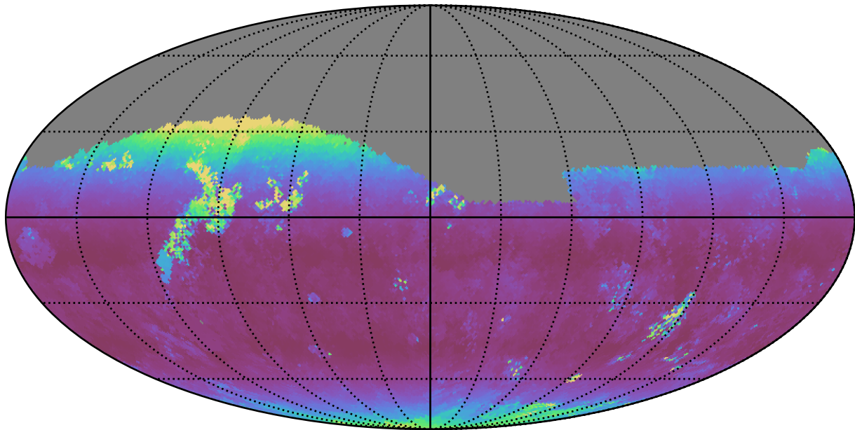
too_elab_r8_d3_gz_v3.4_10yrs Yr 1 z band: Median airmass
