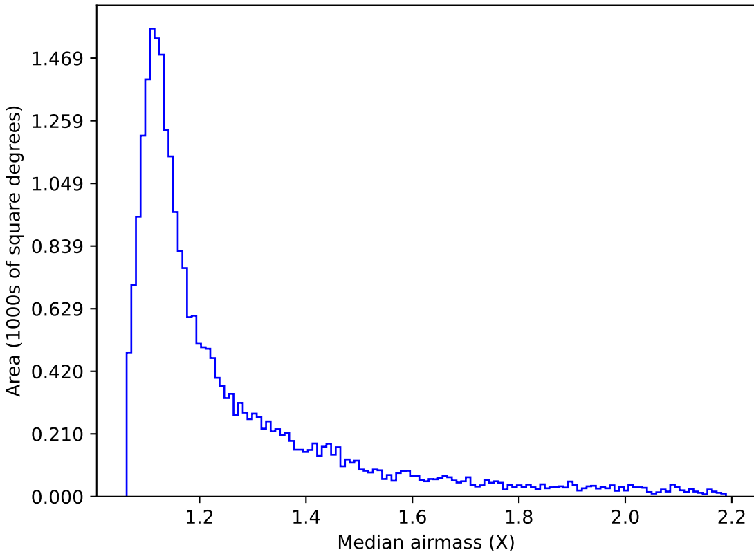
too_elab_r8_d3_gz_v3.4_10yrs Yr 1 z band: Median airmass
