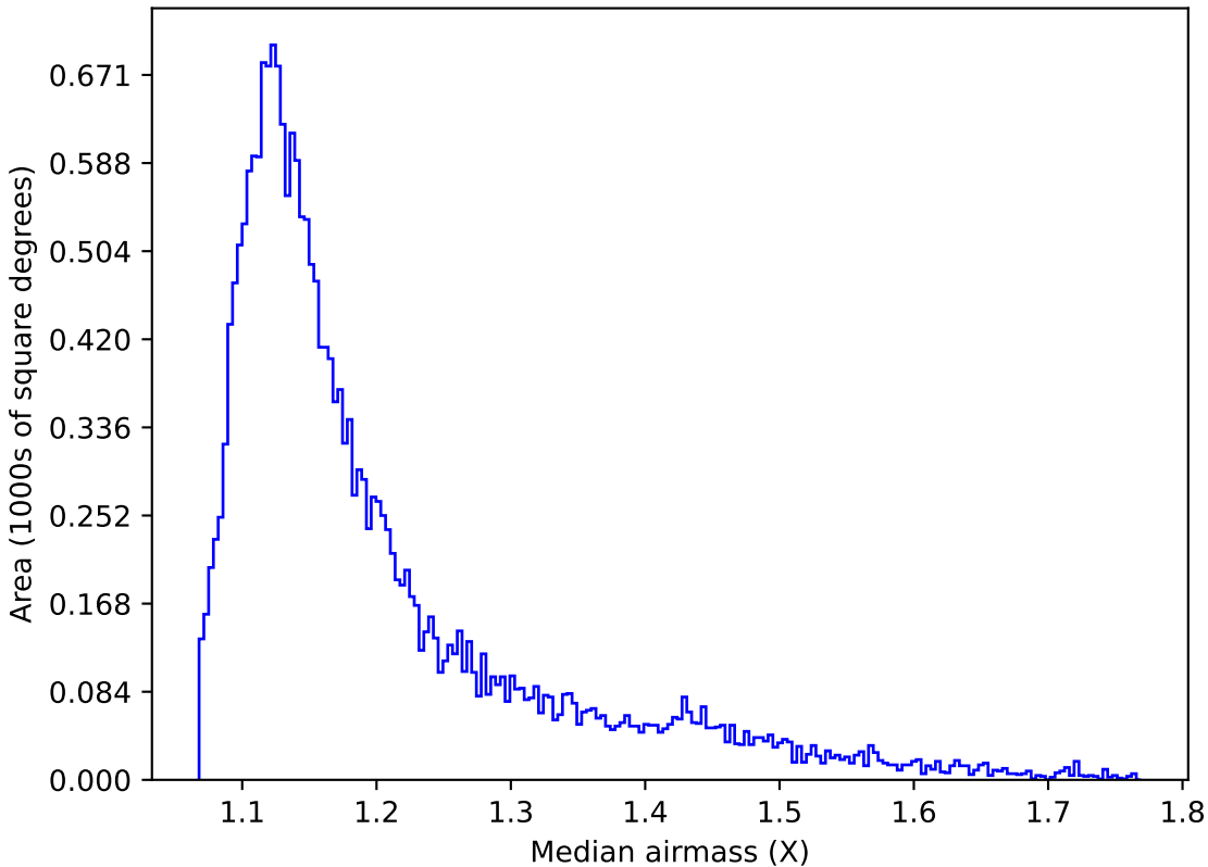
too_elab_r8_d3_gz_v3.4_10yrs Yr 1 y band: Median airmass
