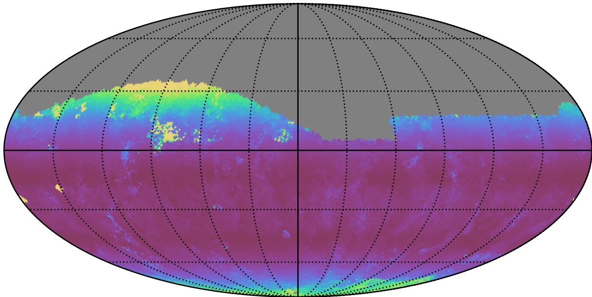
too_elab_r8_d3_gz_v3.4_10yrs Yr 1 i band: Median airmass
