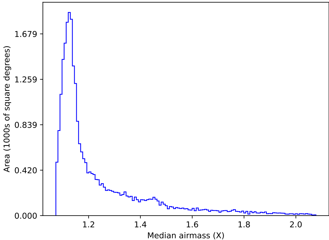
too_elab_r8_d3_gz_v3.4_10yrs Yr 1 all bands: Median airmass
