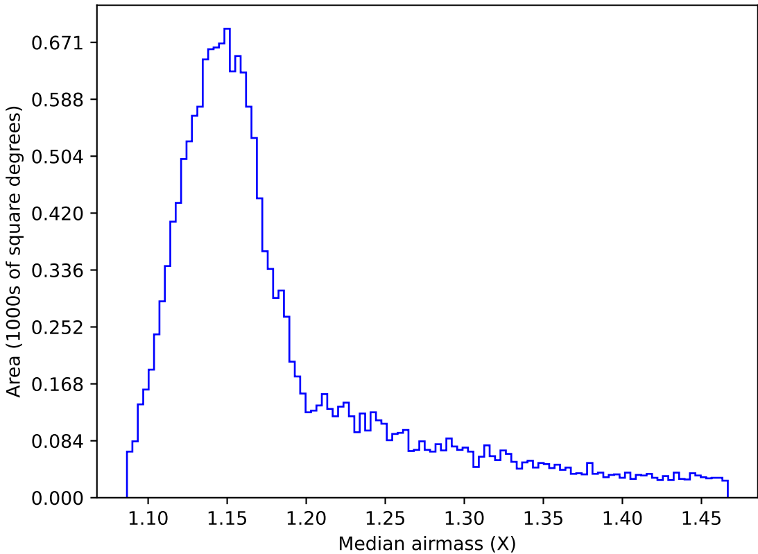
too_elab_r8_d3_gz_v3.4_10yrs WFD z band: Median airmass
