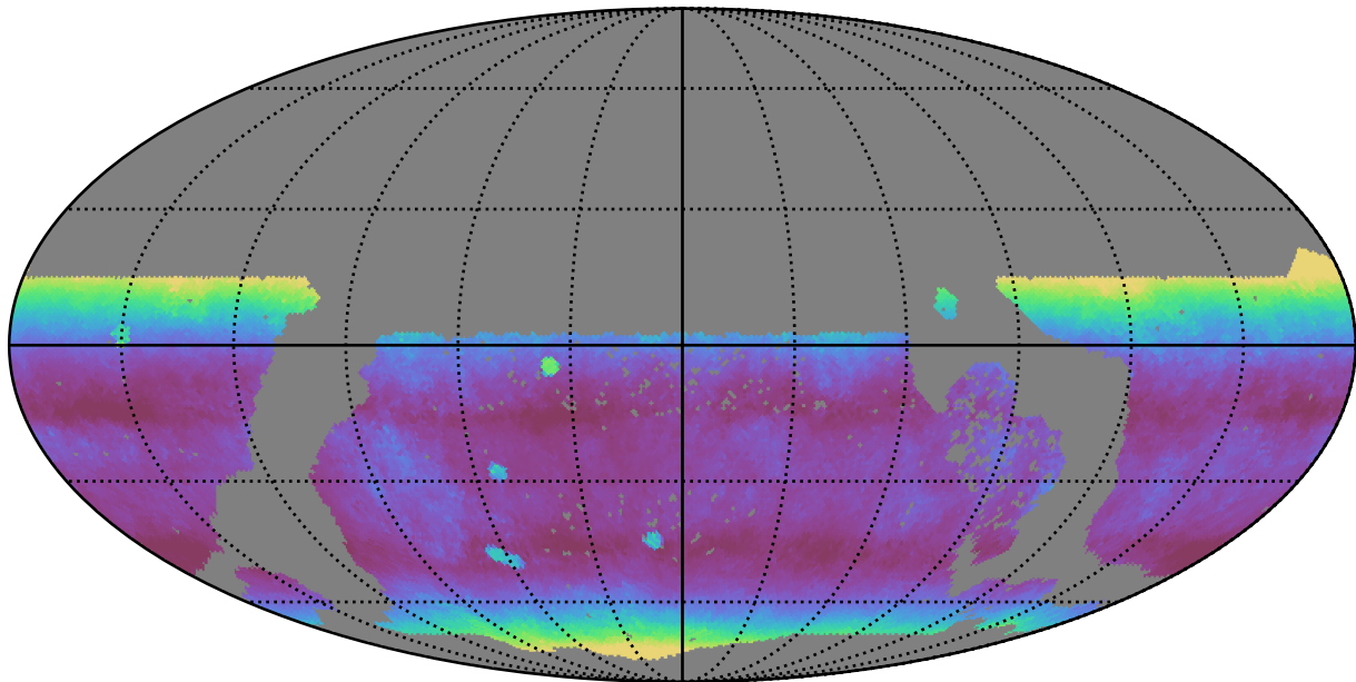
too_elab_r8_d3_gz_v3.4_10yrs WFD y band: Median airmass
