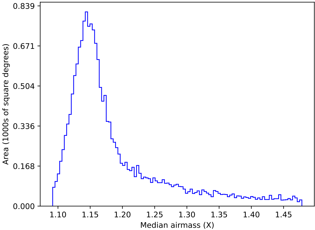
too_elab_r8_d3_gz_v3.4_10yrs WFD y band: Median airmass
