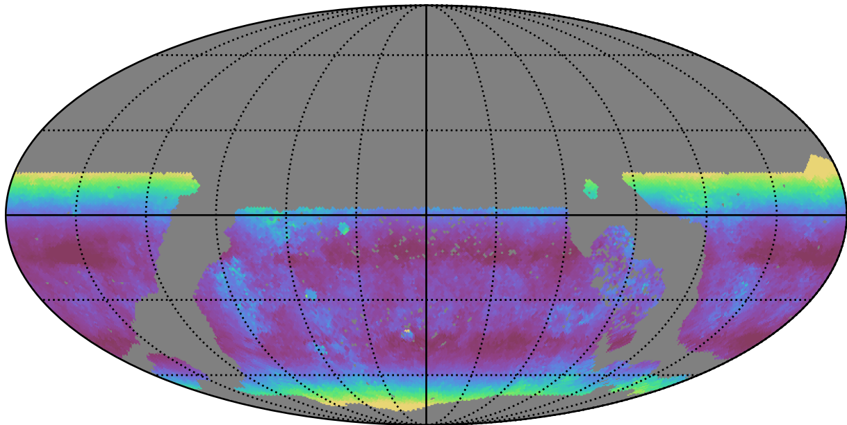
too_elab_r8_d3_gz_v3.4_10yrs WFD u band: Median airmass
